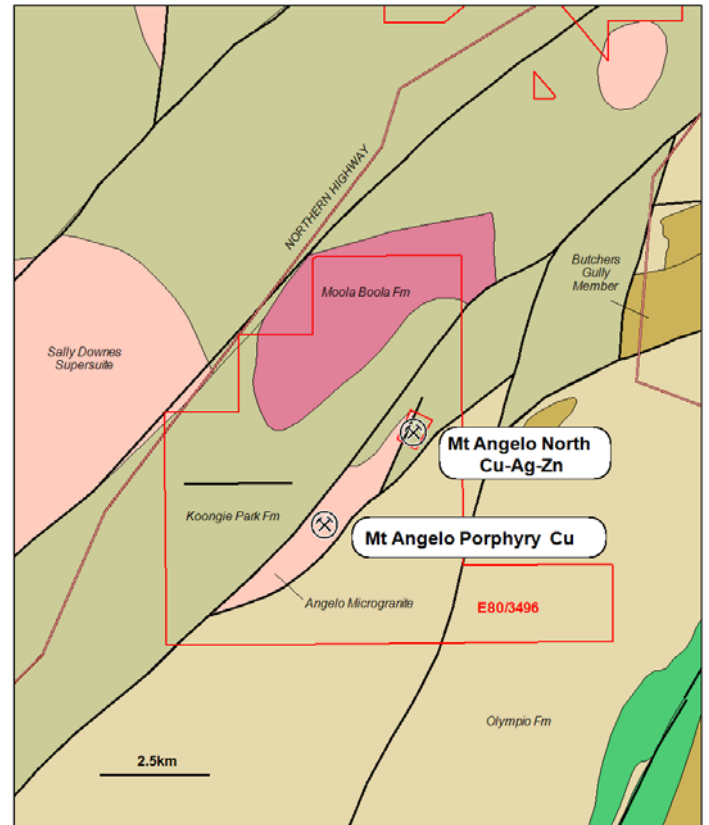
Location and general geology plan
